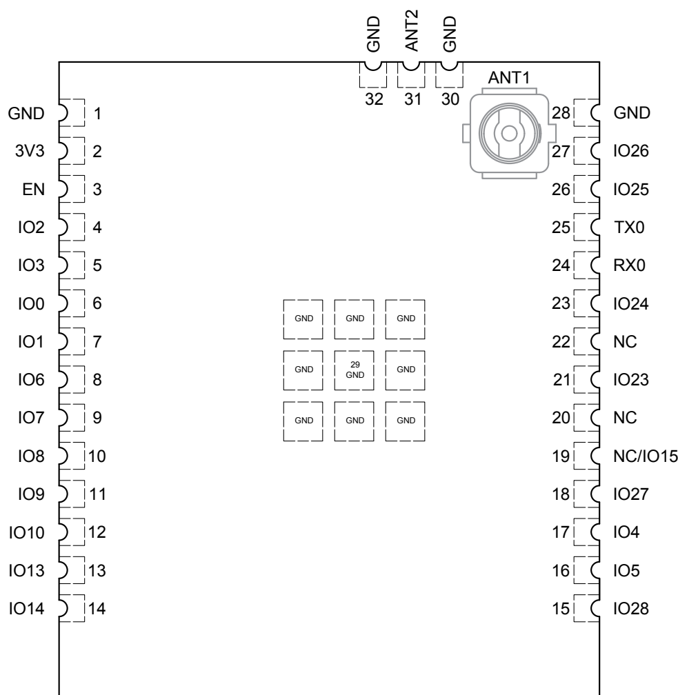
Figure 4: ESP32-C5-WROOM-1U Layout (Top View)
