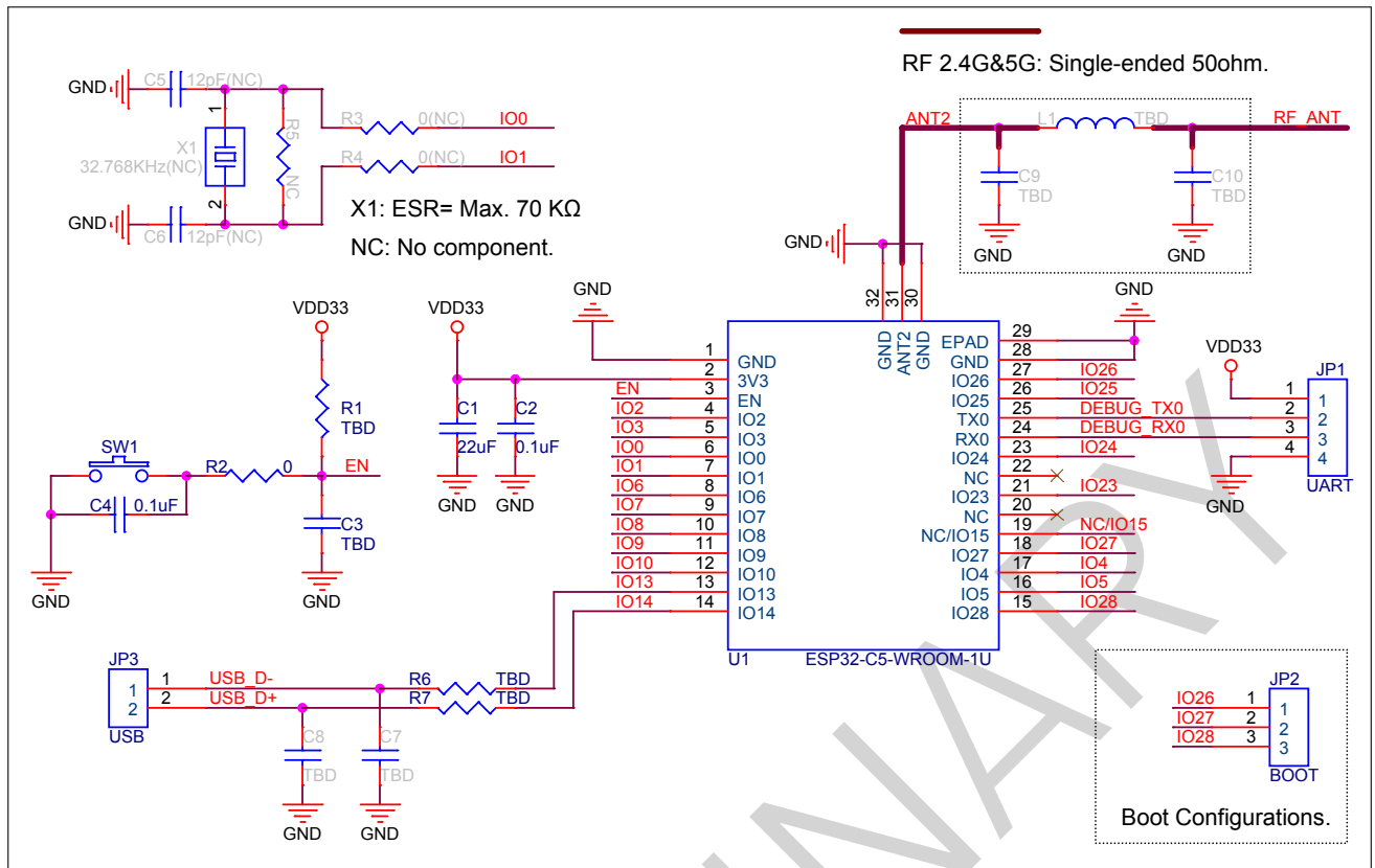
Figure 9: ESP32-C5-WROOM-1U Schematics
