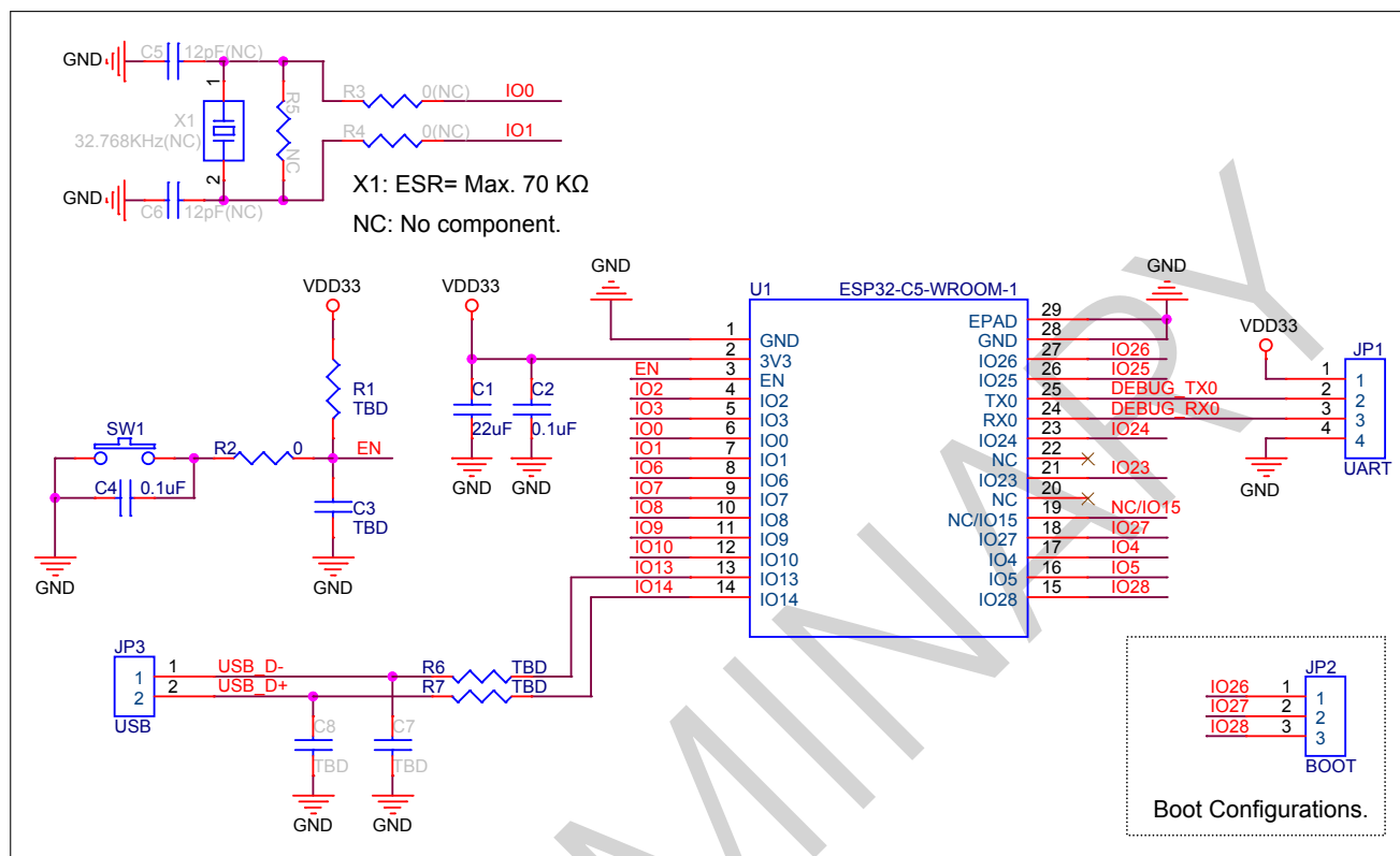
Figure 8: ESP32-C5-WROOM-1 Schematics
