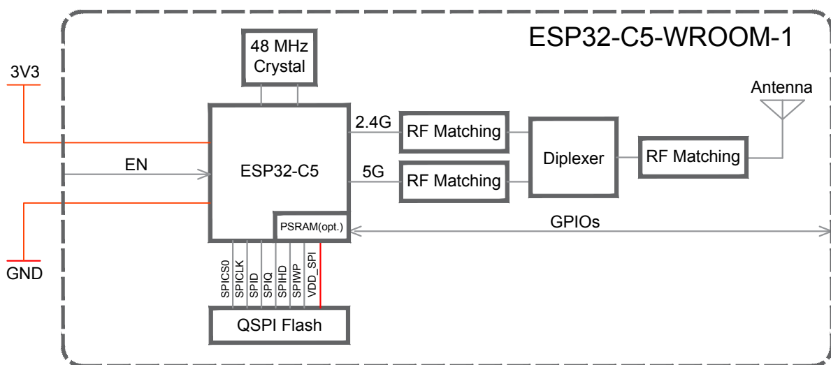
Figure 1: ESP32-C5-WROOM-1 Block Diagram
