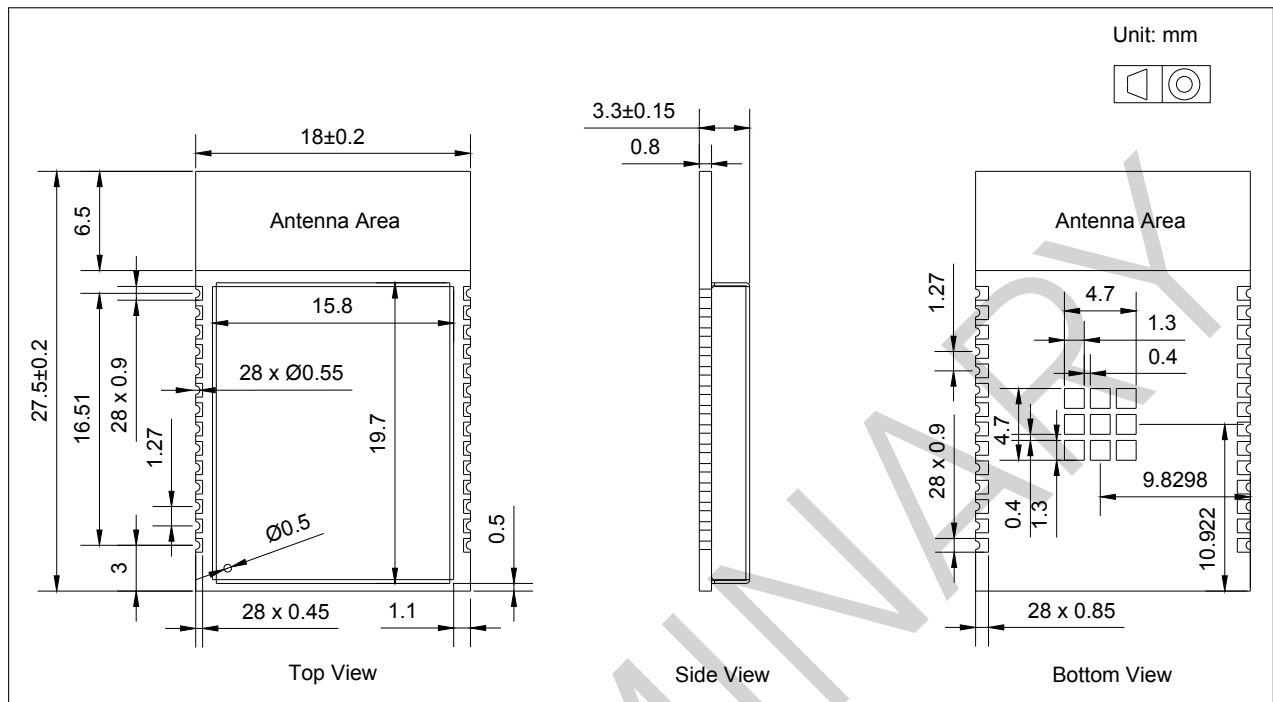
Figure 10: ESP32-C5-WROOM-1 Dimensions
