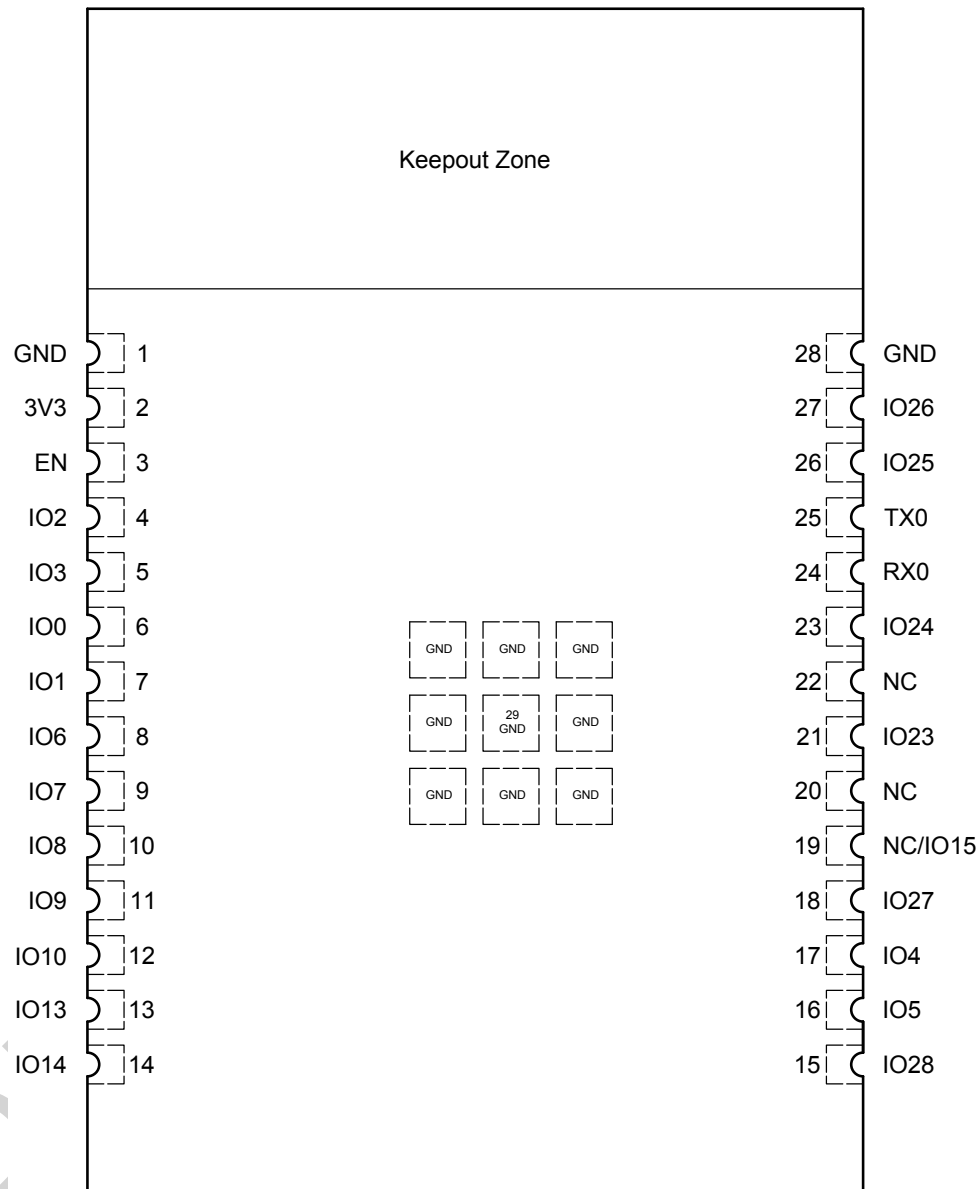
Figure 3: ESP32-C5-WROOM-1 Layout (Top View)
