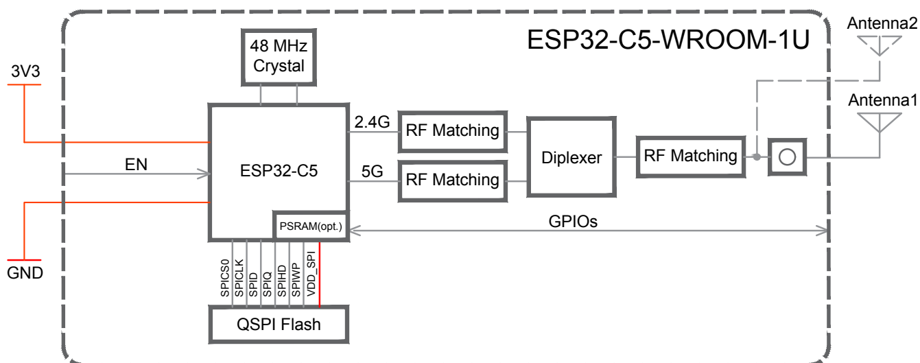
Figure 2: ESP32-C5-WROOM-1U Block Diagram
