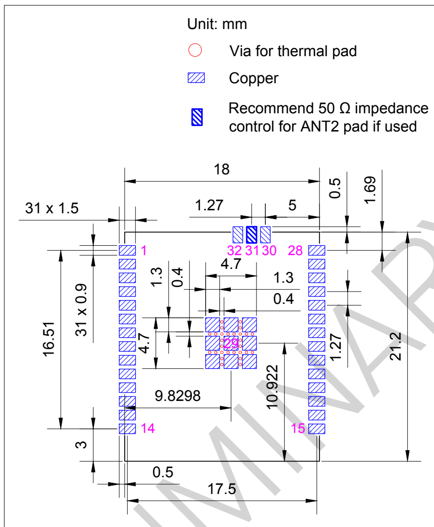
Figure 14: ESP32-C5-WROOM-1U PCB Land Pattern
