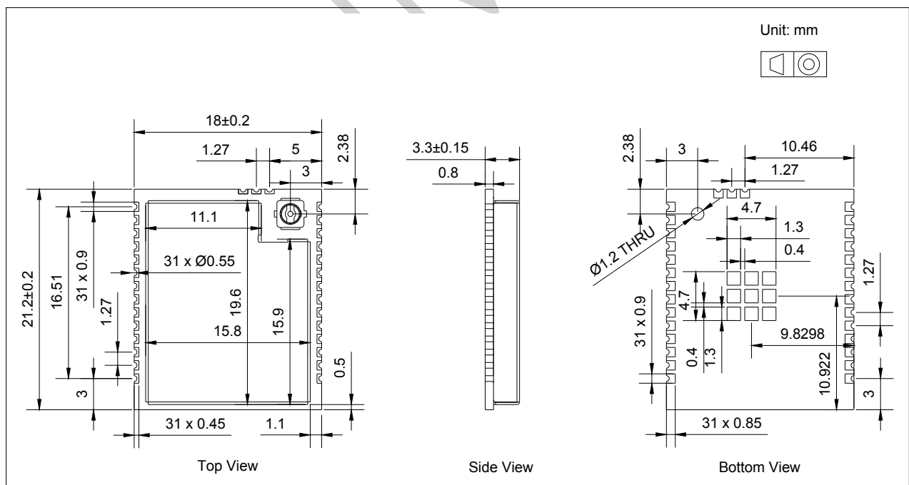
Figure 11: ESP32-C5-WROOM-1U Dimensions
