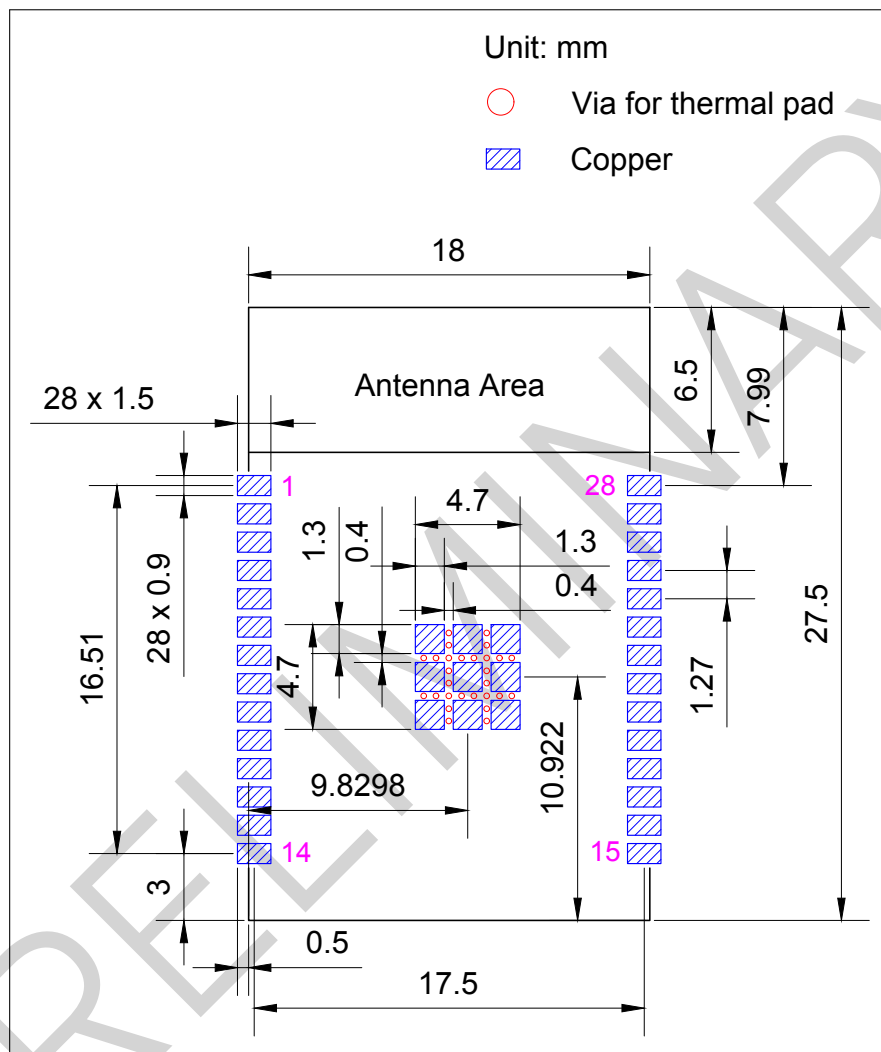
Figure 13: ESP32-C5-WROOM-1 PCB Land Pattern
