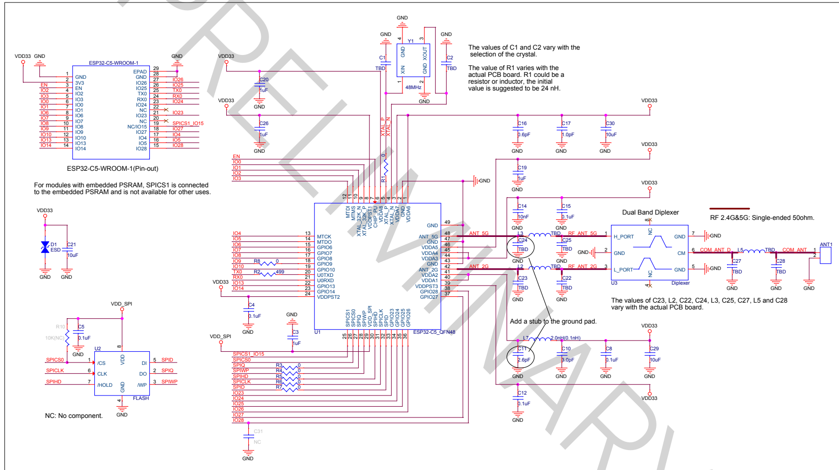
Figure 6: ESP32-C5-WROOM-1 Schematics
